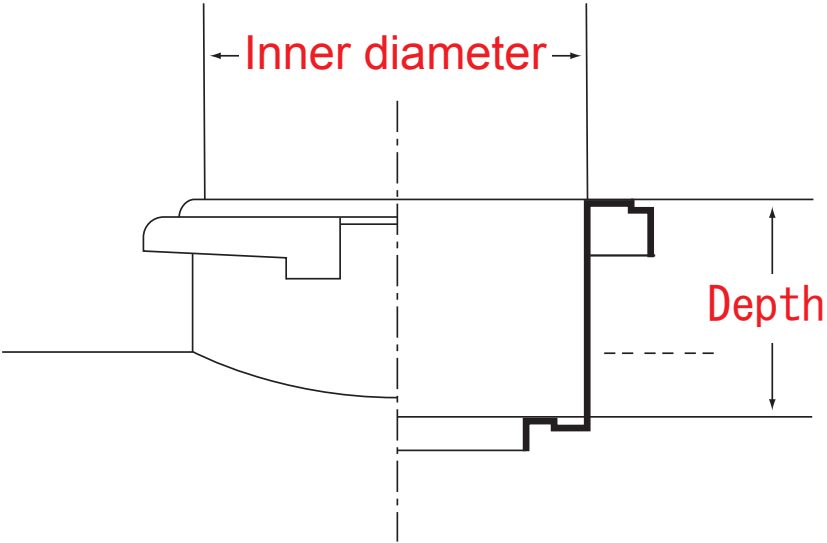
For filler neck of current vehicle (hook-type)
