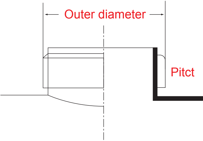
For filler neck of current vehicle (Screw-type)
